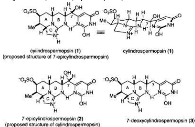
Figure 2: Proposed 7-epicylindrospermopsin and CYN Structures
