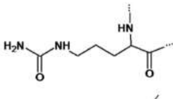
Figure 6: Ureido Group (from a citrullin residue)
