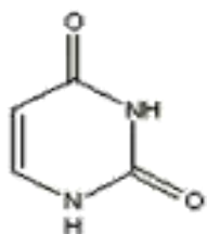
Figure 5: Free Uracil Group
