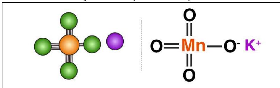
Figure 4: Structure of Potassium Permanganate
