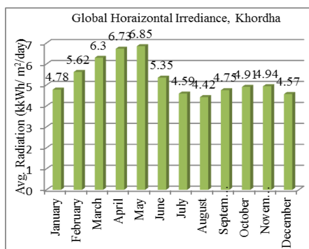
Fig. 3: Monthly global horizontal irradiance of Khordha, Odisha
